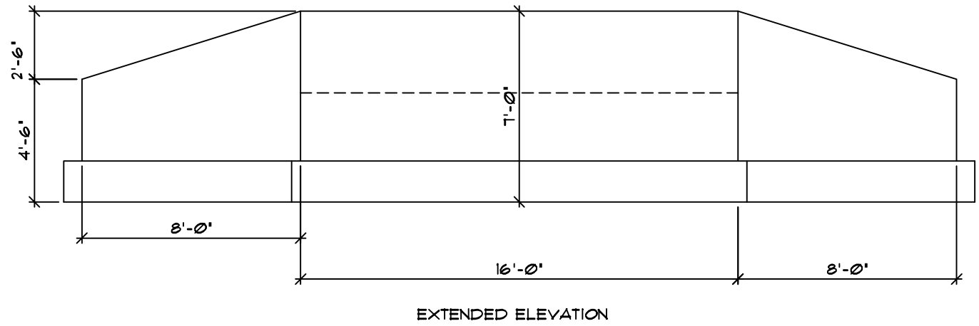
BRIDGE ABUTMENT DETAILS
